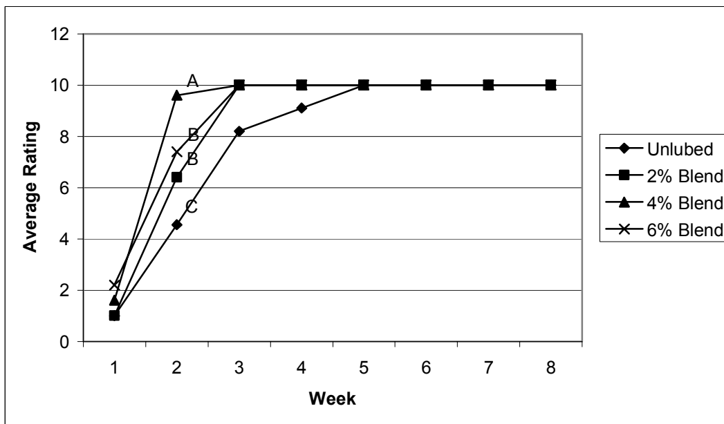
Figure 3: Comparison of average weekly mold ratings for 70% wood content WPCs containing zinc stearate lubricant at 2, 4, and 6% loadings. Means with the same letter designation at the 3 week exposure time are not significantly different at the 95% confidence level.
