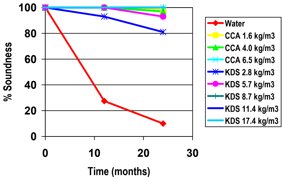
Graph 19: Field Stake termite Test Saucier
