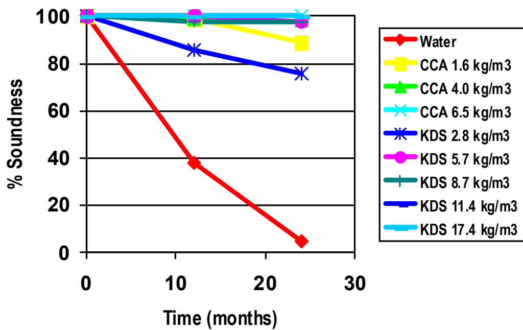
Graph 15: Field Stake Test - Saucier, MS
