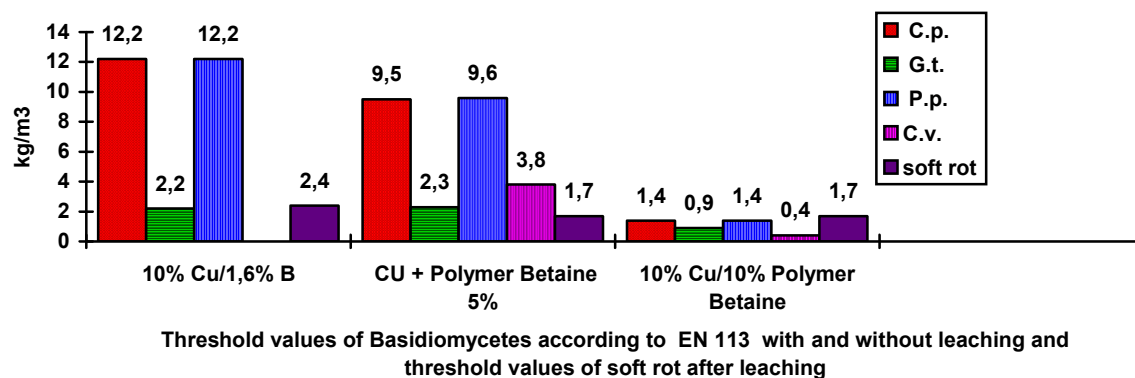
Graph 10: Comparision: Efficacy of Copper/Amine-formulations
